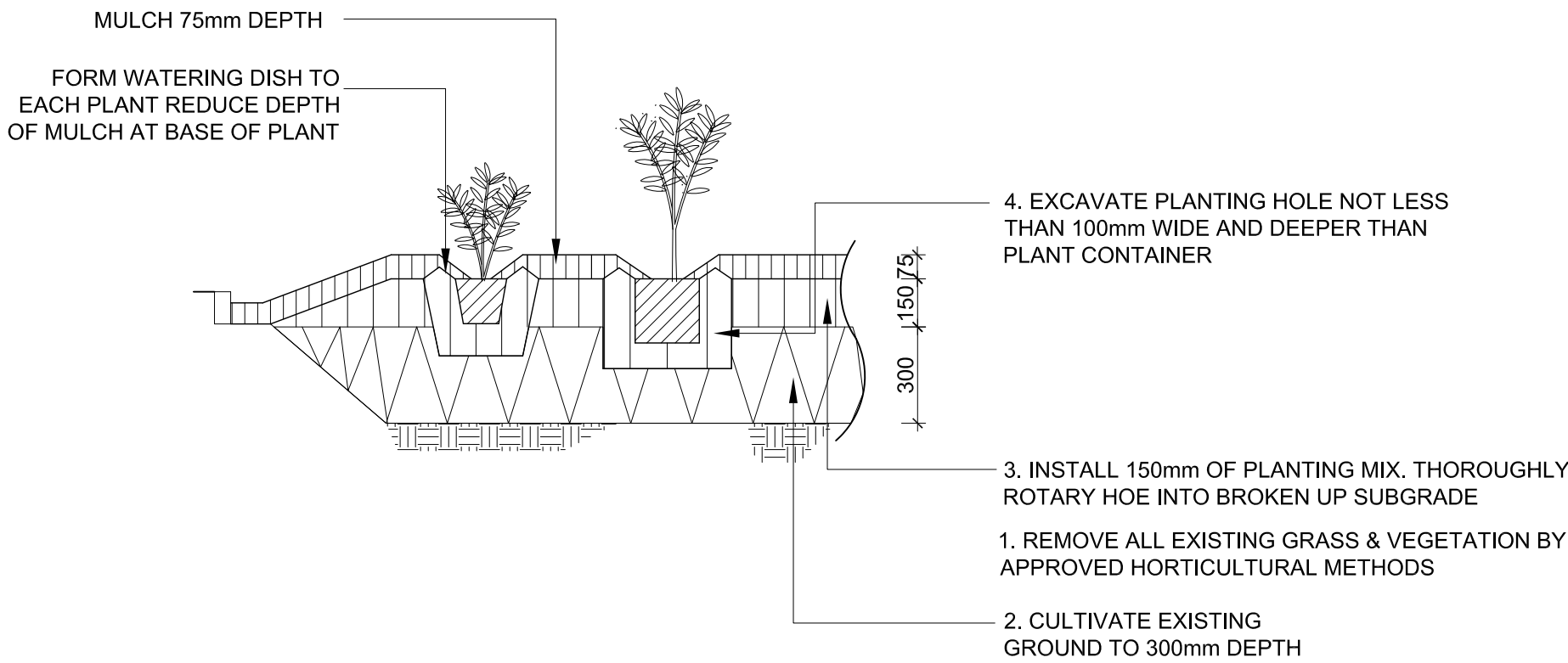
2 MASS PLANTING BED-NATURAL GROUND TYPICAL SECTION 1:20
