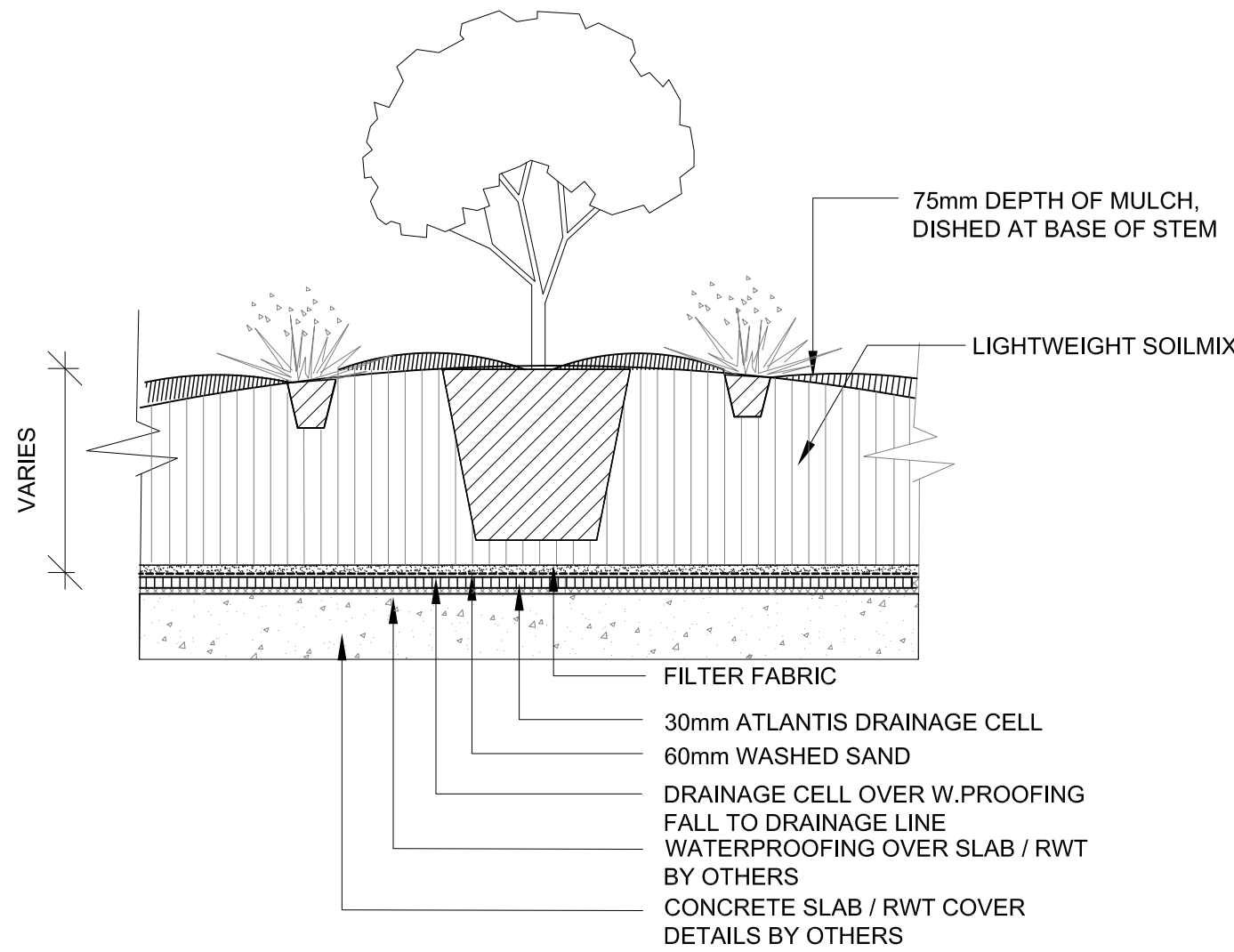
3 ON-SLAB PLANTING DETAIL SCALE 1:20
